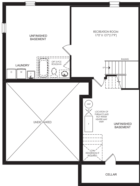
BASEMENT EL. A & B
