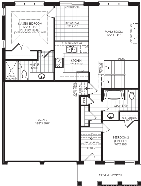
GROUND FLOOR EL. A
