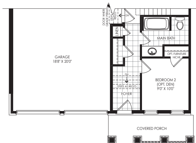
PARTIAL GROUND FLOOR EL. B
