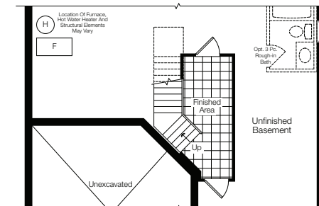
Partial Basement Floor For Opt. Loft Condition
