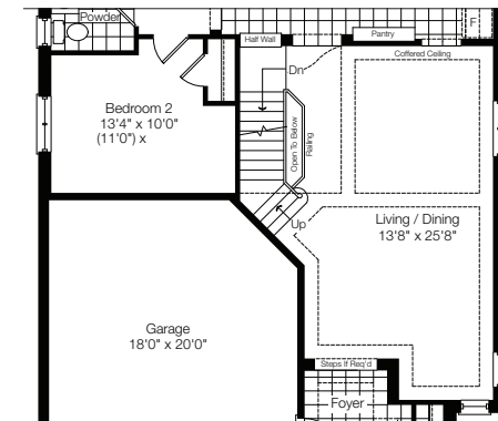
Partial Ground Floor Elev. 'A' & 'B' For Opt. Loft
